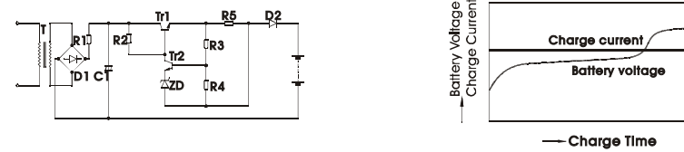
Figure11 CONSTANT CURRENT CHARGE CIRCUIT CONSTANT CURRENT CHARGE CHARACTERISTIC
